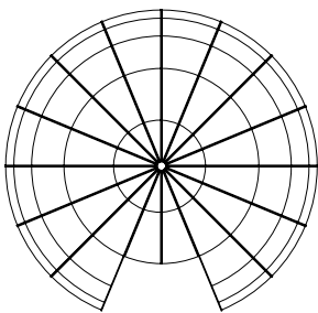
IGLOO Ø3760 x h:2520 mm
