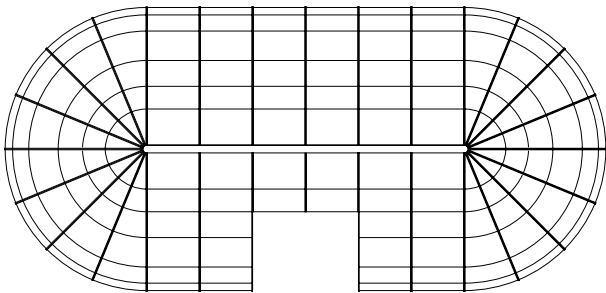
IGLOO SYSTEM (Beispielkonfiguration / example configuration) 7960 x 3760 x h:2520 mm
