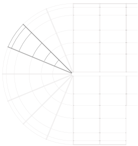
IGLOO UNIT 1 733.5 x 1827.5 x h:2520 mm
